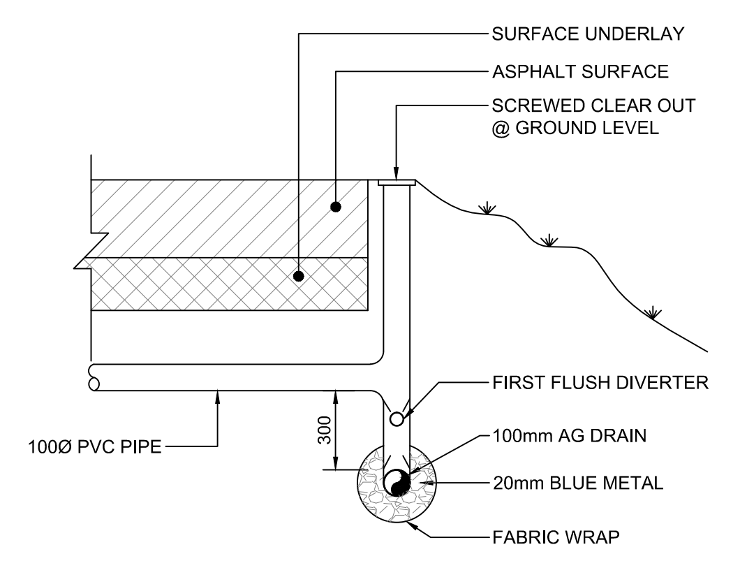
DETAIL AA - CLEAR OUT AND SUB SOIL DRAINAGE NTS
